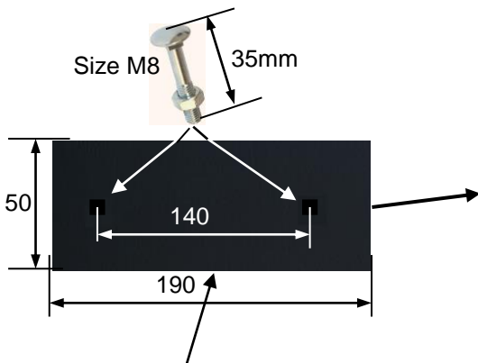
Metal backplate including two special bolts and nuts. See below the instruction of use.
