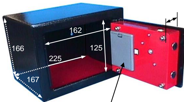
Battery holder ( 4xAA battery) Remove cover to place batteries
